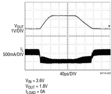
VOUT Short to VIN (Forced Continuous Mode)
