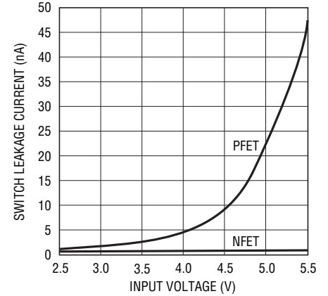
Switch Leakage Current vs Input Voltage
