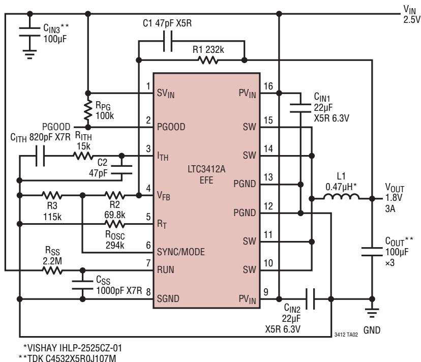
1.8V, 3A Step-Down Regulator at 1MHz, Burst Mode Operation
