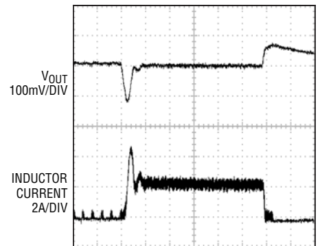
Load Step Transient Burst Mode Operation
