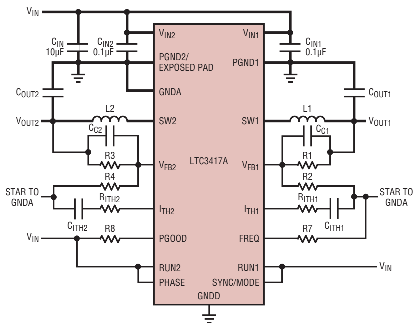
Figure 5. Layout Guideline
