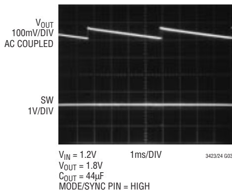
Burst Mode Operation at 500μA Load
