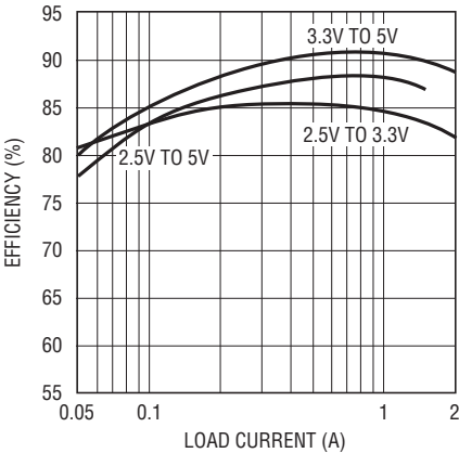
Converter Efficiency
