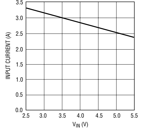
Peak Current Clamp vs V_{IN}
