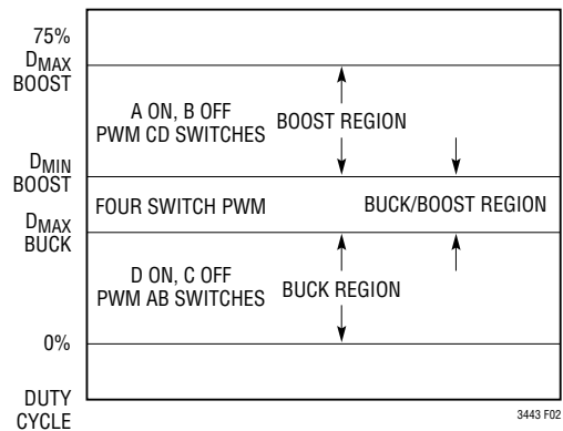
Figure 2. Switch Control vs Internal Control Voltage, V_{CI}
