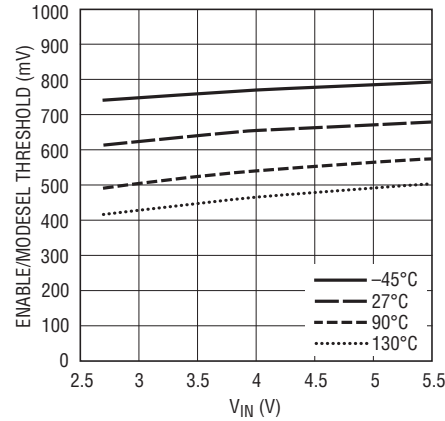
Enable/MODESEL Thresholds
