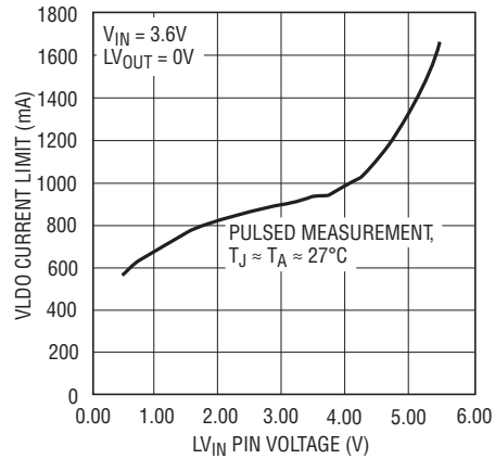
VLDO Current Limit vs V_{IN} Voltage
