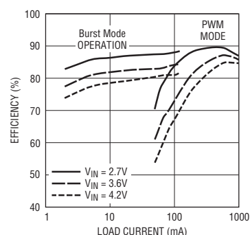
Buck Efficiency vs Buck Load Current
