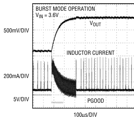
Figure 5. Transition from DAC = MIN to DAC = MAX
