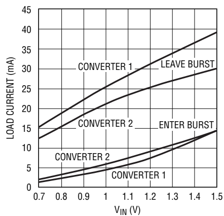
Burst Mode Threshold Current vs V_{IN} for V_{OUT1} = V_{OUT2} = 1.8V
