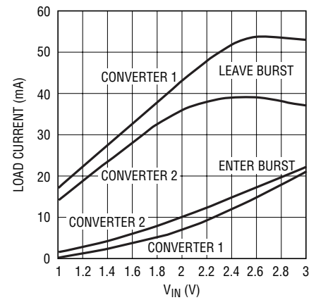
Burst Mode Threshold Current vs V_{IN} for V_{OUT1} = V_{OUT2} = 3.3V
