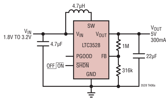
2 Cell to 5V
