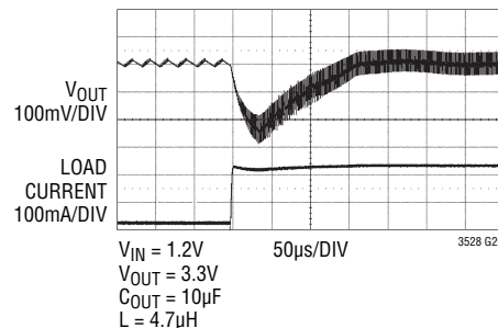
Load Step Response (Burst Mode Operation, 1.2V to 3.3V, LTC3528)
