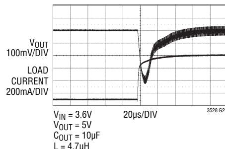
Load Step Response (Fixed Frequency, 3.6V to 5V)
