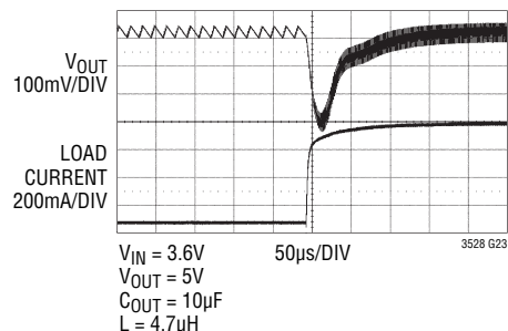
Load Step Response (Burst Mode Operation, 3.6V to 5V, LTC3528)
