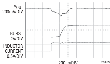
Transition from Burst Mode Operation to Fixed Frequency Mode
