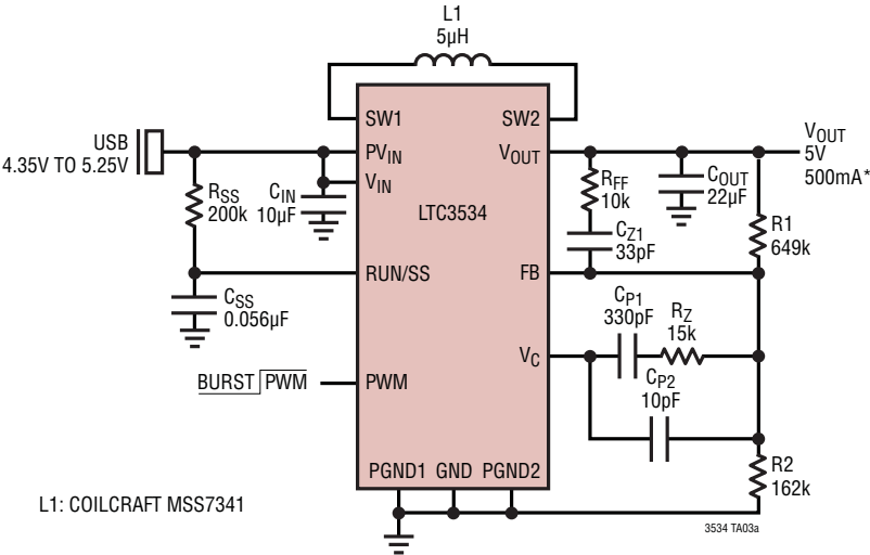
USB to 5V at 500mA
