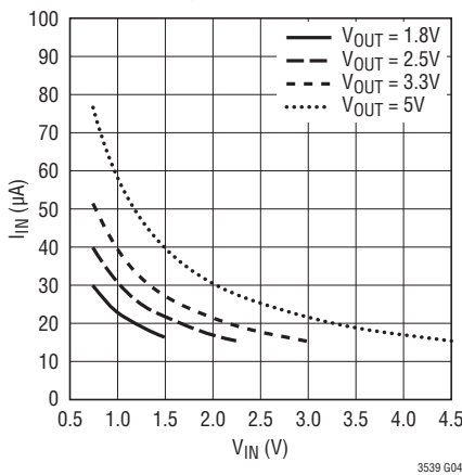
No Load Input Current vs V_{IN}
