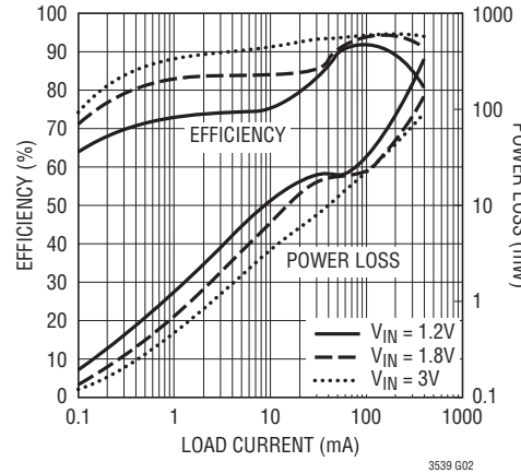
Efficiency vs Load Current and V_{IN} , V_{OUT} = 3.3\text{V}
