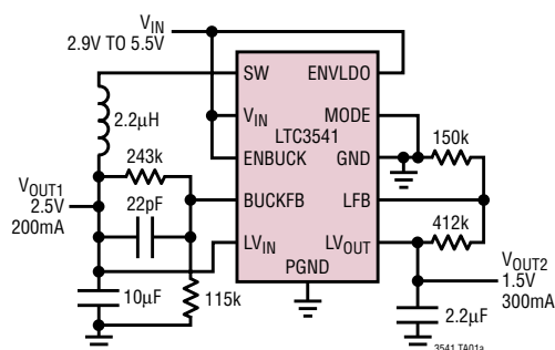
LTC3541 Typical Application
