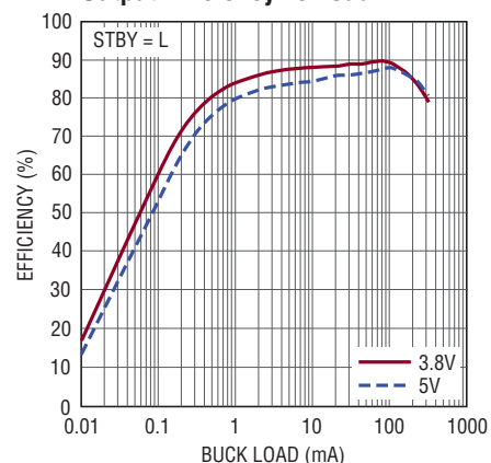
Buck Switching Regulator 1.8V Output Efficiency vs Load
