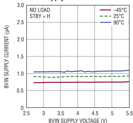
Buck Regulator Standby Mode BVIN Supply Current
