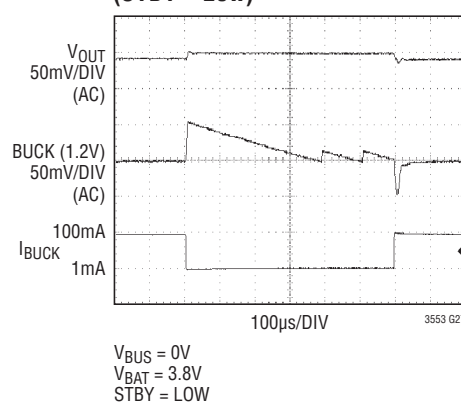
Buck Regulator Output Transient (STBY = Low)
