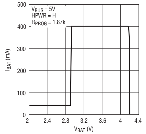
I_{BAT} vs V_{BAT} (LTC3554/LTC3554-2)
