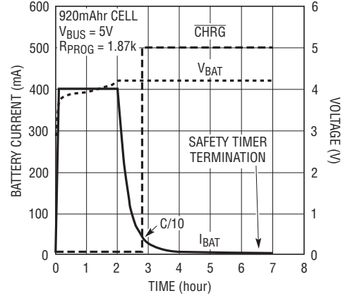
Battery Charge Current and Voltage vs Time (LTC3554/LTC3554-2)
