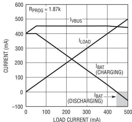
V_{BUS} and Battery Current vs Load Current
