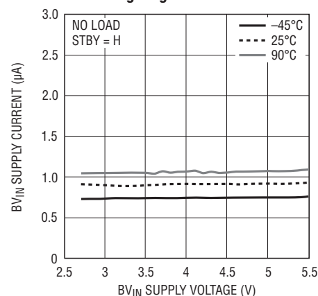
Standby Mode BV IN Supply Current Per Enabled Step-Down Switching Regulator
