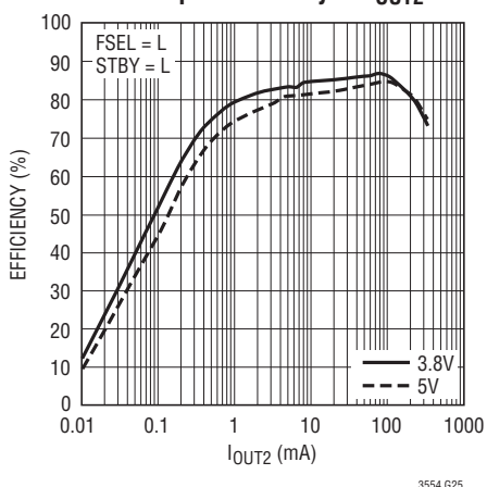
Step-Down Switching Regulator 2 1.2V Output Efficiency vs I OUT2
