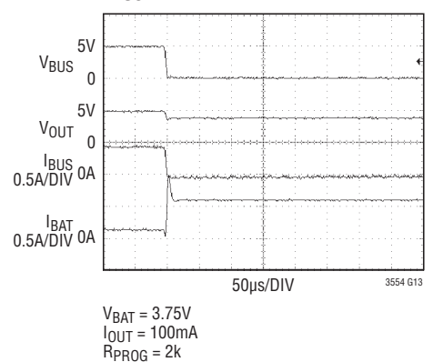
V_{BUS} Disconnect Waveform
