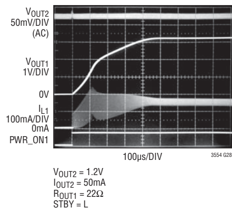
Step-Down Switching Regulator Start-Up Waveform
