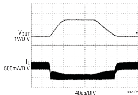
V_{OUT} Short to V_{IN} (Forced Continuous Mode)
