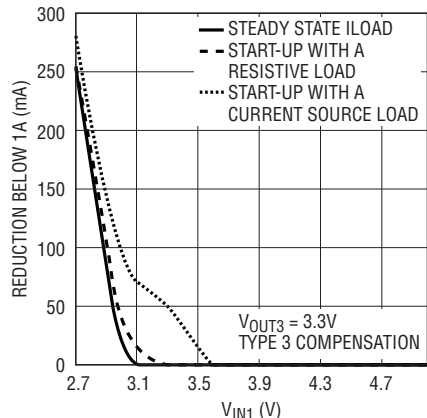
Reduction in Current Deliverability at Low V_{IN1}
