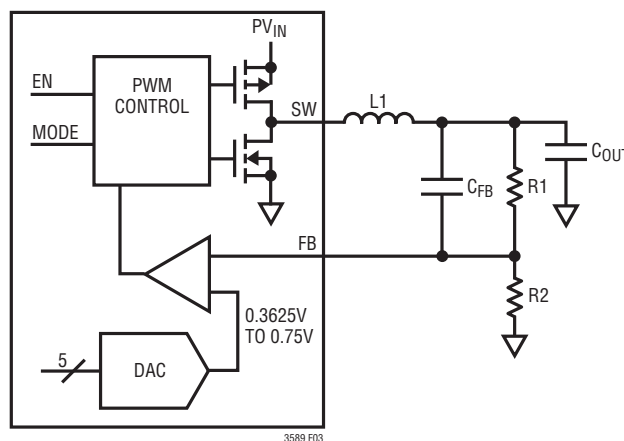
Figure 3. Step-Down Switching Regulator Application Circuit
