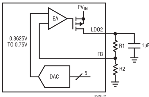
Figure 2. LD02 Application Circuit
