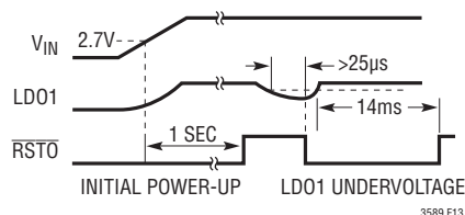
Figure 13. Initial Power-Up and LDO1 Undervoltage \overline{RSTO} Timing
