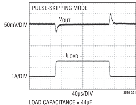
Step-Down Switching Regulator 1 Load Step
