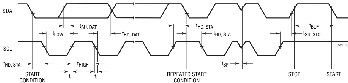
Figure 18. LTC3589/LTC3589-1 I 2 C Timing
