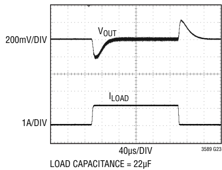
Buck-Boost Switching Regulator 1 Load Step
