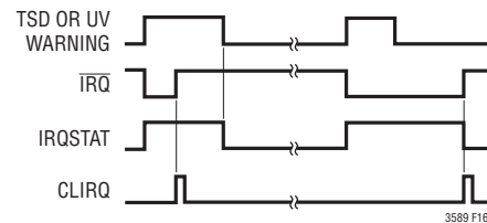
Figure 16. \overline{IRQ} and IRQSTAT Status Register Warning Timing
