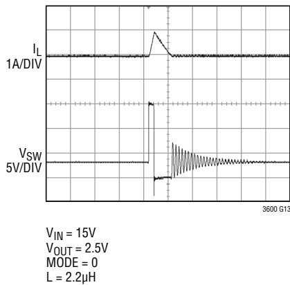
Discontinuous Conduction Mode Operation
