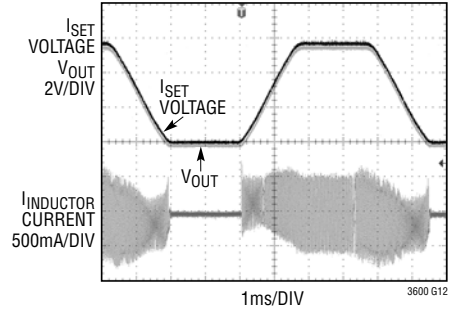
Output Tracking
