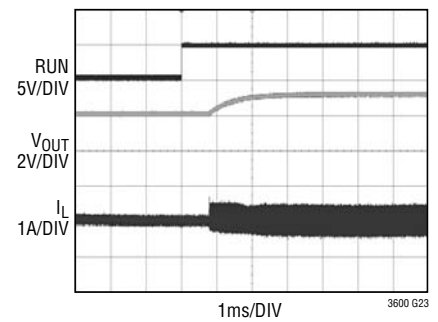
Start-Up Waveform
