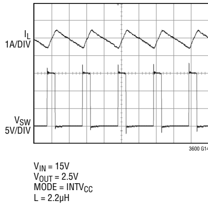
Continuous Conduction Mode Operation
