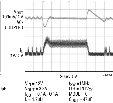
Transient Response DCM, Operation, Internal Compensation
