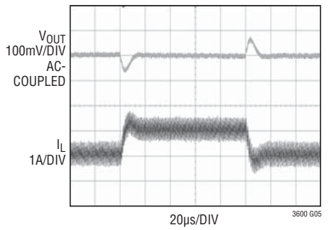
Transient Response CCM Operation, External Compensation
