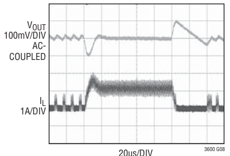
Transient Response DCM, Operation, Internal Compensation
