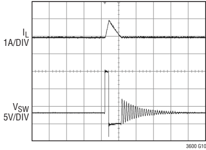
DCM Operation
