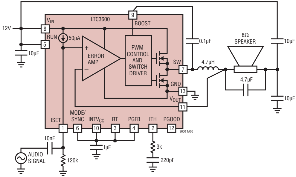
High Efficiency 12V Audio Driver
