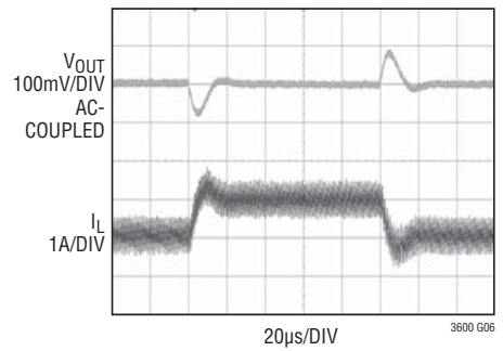
Transient Response CCM Operation, Internal Compensation
