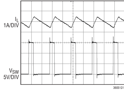
CCM Operation
