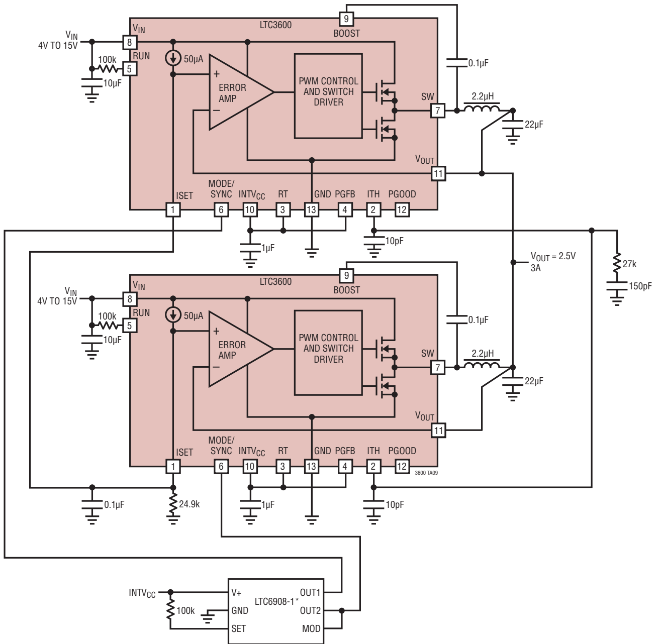
15V, 3A Dual Phase Single-Output Regulator
