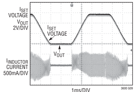
Output Tracking
