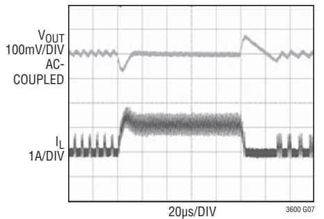
Transient Response DCM, Operation, External Compensation
