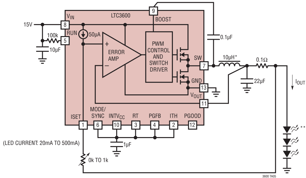
LED Driver with Programmable Dimming Control
