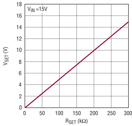
V SET vs R SET
