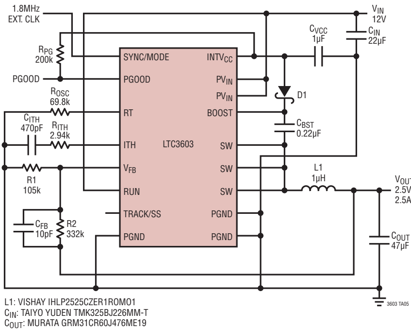
3.3V, 2.5A Regulator, Synchronized to 1.8MHz, Small Size
