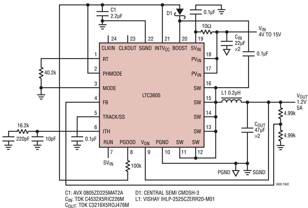
12V to 1.2V 4MHz Buck Regulator
