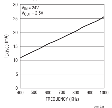
I_{\text{EXTVCC}} vs Frequency
