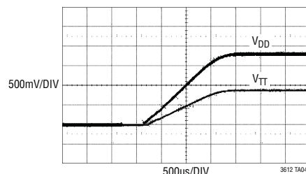
Ratiometric Start-Up
