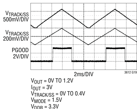
Tracking Up/Down in Forced Continuous Mode, DDR Pin Tied to SV_{IN}
