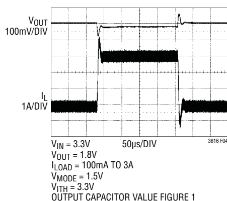
Figure 4. Load Step Transient Forced Continuous Mode with AVP Mode
