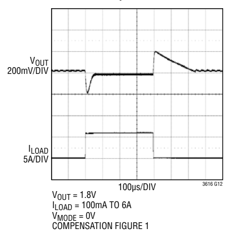
Load Step Transient in Burst Mode Operation
