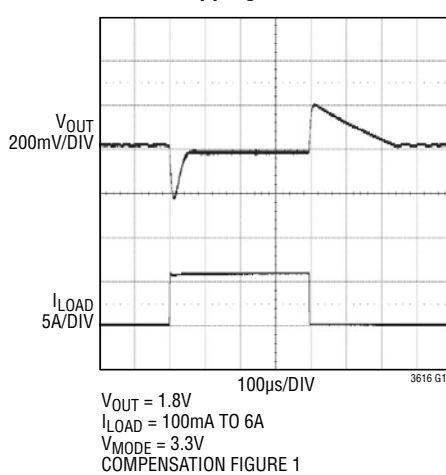
Load Step Transient in Pulse-Skipping Mode
