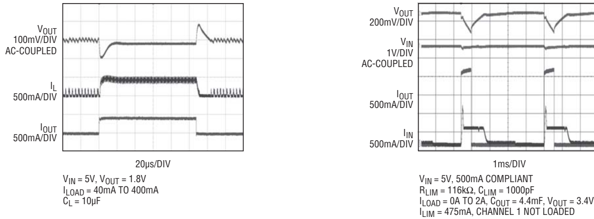
Figure 4c. Transient Response
