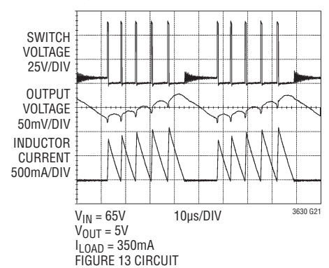
Operating Waveforms
