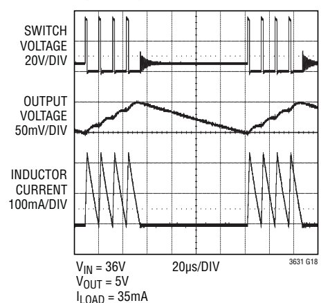
Operating Waveforms
