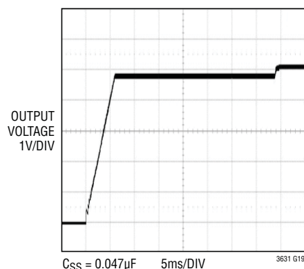
Soft-Start Waveform
