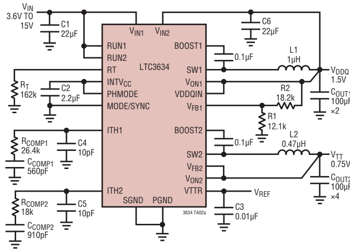
Figure 12a. V_{TT} Powered from V_{DDQ}
