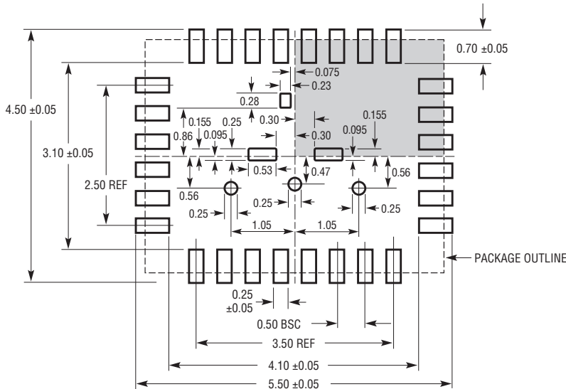
UFD Package 28-Lead Plastic QFN (4mm × 5mm) (Reference LTC DWG # 05-08-1538 Rev A) Exposed Pad Variation AA
