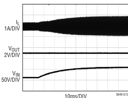
Output Regulation with V_{IN} Slew
