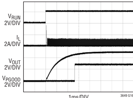
Start-up Waveform
