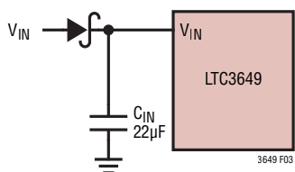
Figure 3. Schottky Diode in Series with the Supply
