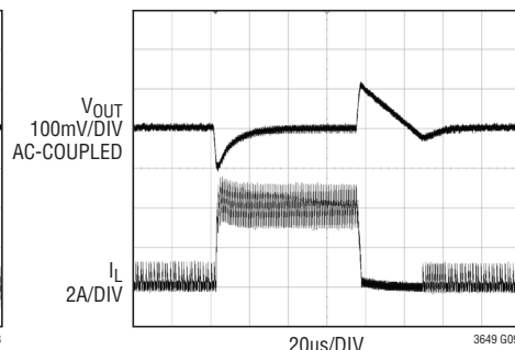
Transient Response, Burst Mode
