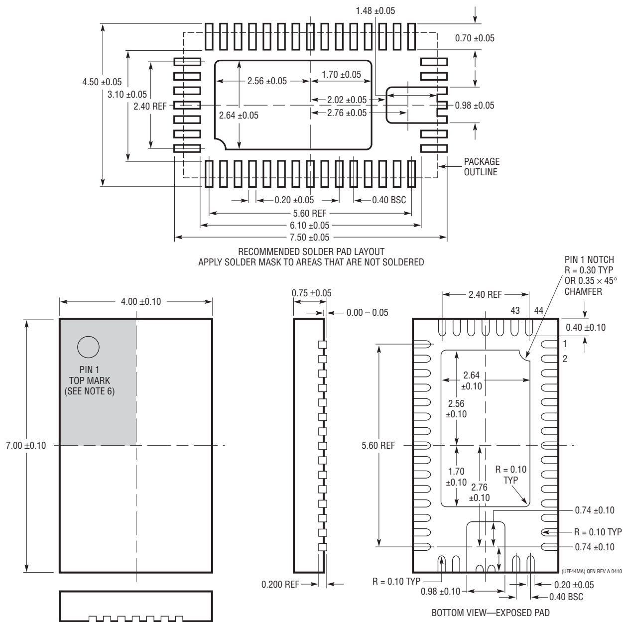
UFFMA Package 44-Lead Plastic QFN (4mm × 7mm) (Reference LTC DWG # 05-08-1762 Rev A)
