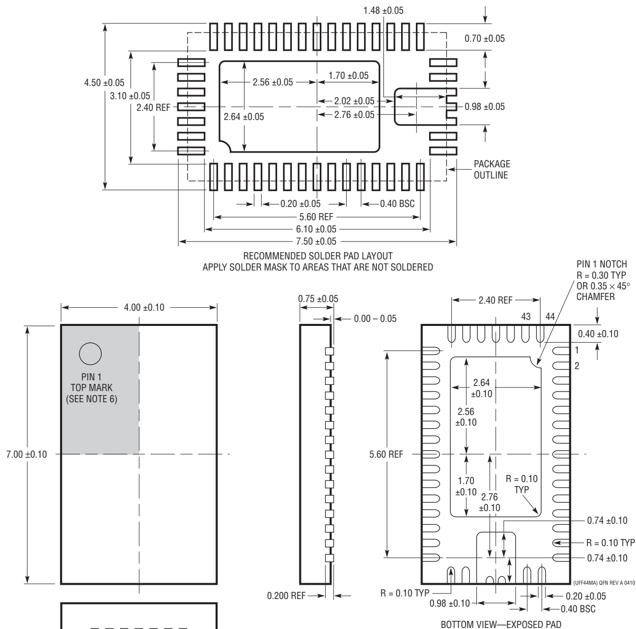
UFF Package Variation: UFF44MA 44-Lead Plastic QFN (4mm × 7mm) (Reference LTC DWG # 05-08-1762 Rev A)
