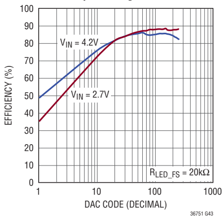
LED Driver, Dual String Efficiency, 10 LEDs per String
