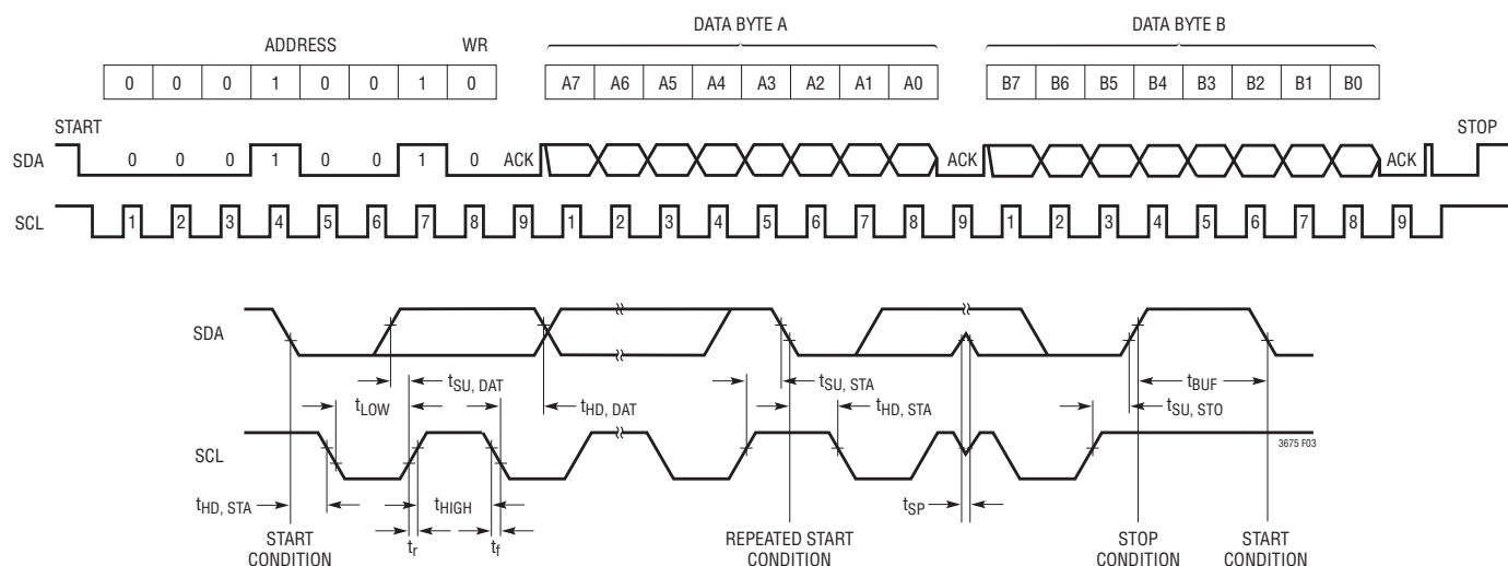
Figure 3. I 2 C Bus Operation
