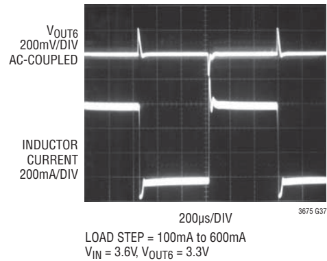
Buck-Boost Regulator Transient Response (PWM Mode)
