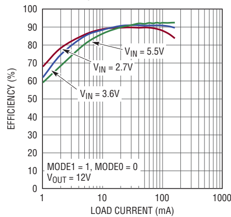
High Voltage Boost Regulator, Efficiency vs Load
