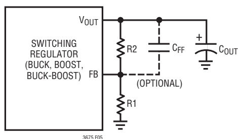
Figure 5. Feedback Components
