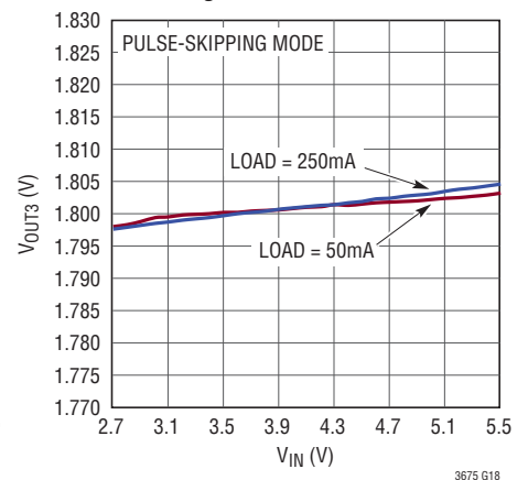
500mA Buck Regulators, Line Regulation
