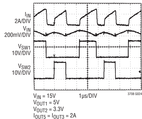
2-Phase Operation
