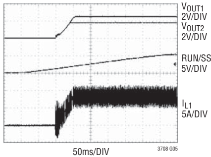
Soft-Start
