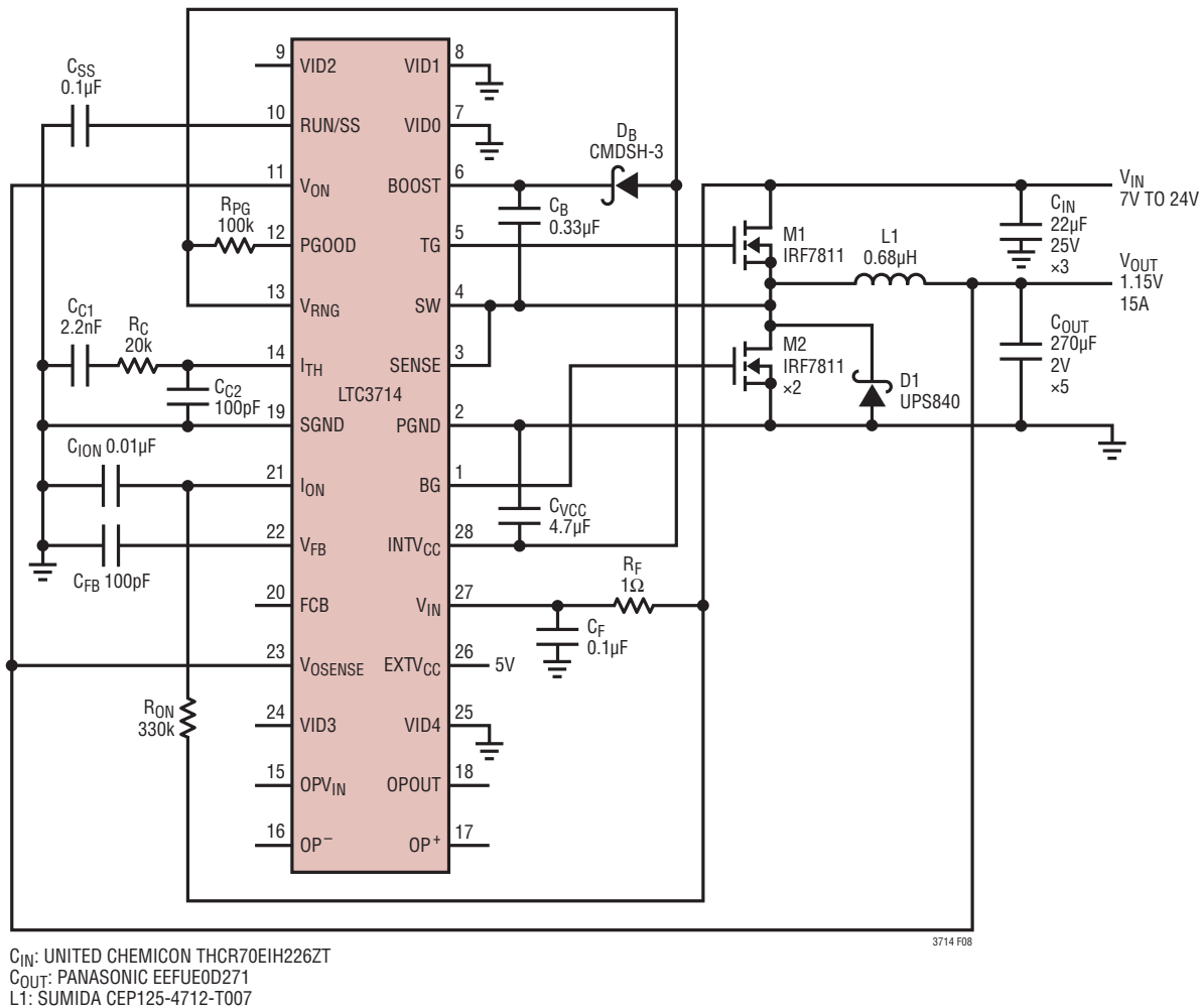
Figure 8. CPU Core Voltage Regulator 1.15V/15A at 300kHz without Active Voltage Positioning
