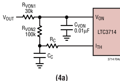
Figure 4. Correcting Frequency Shift with Load Current Changes
