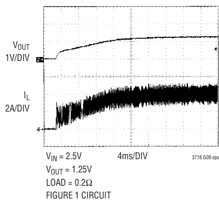
Start-Up Response
