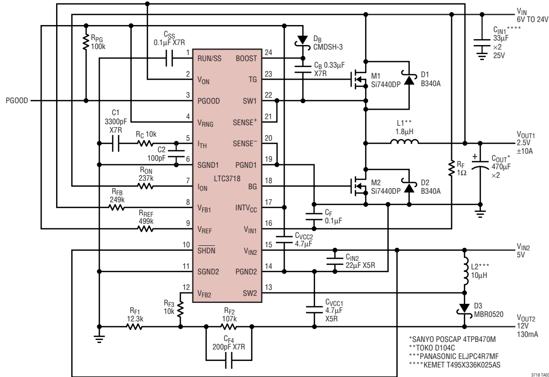
Dual Output 2.5V, \pm 10A Buck Converter and 5V to 12V/130mA Boost Converter
