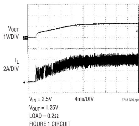
Start-Up Response
