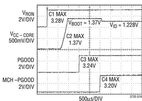
Start-Up Sequence (Figure 14)
