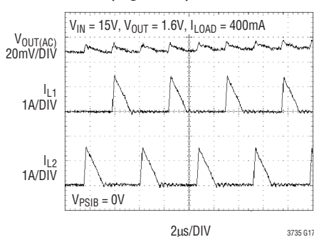
Constant Frequency Low Current Mode (Figure 14)
