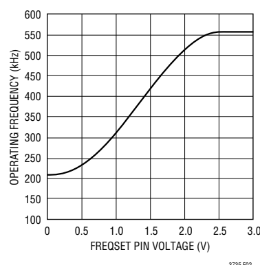
Figure 2. Operating Frequency vs V_{FREQSET}
