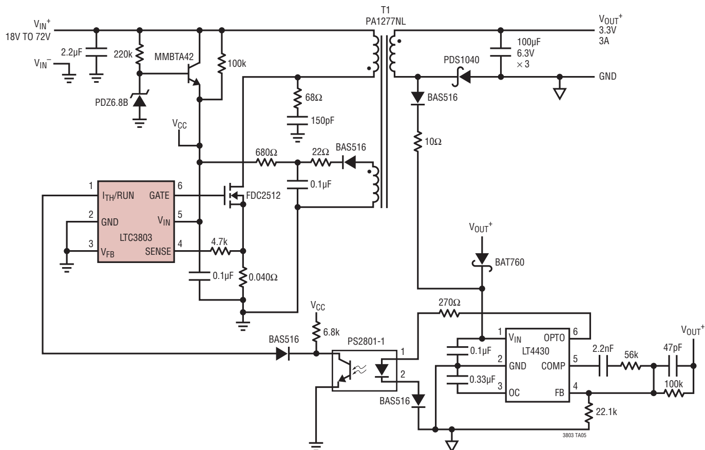
4:1 Input Range 3.3V Output Isolated Flyback DC/DC Converter
