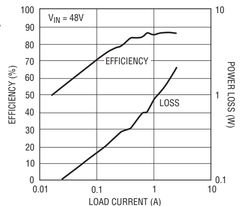
Efficiency and Power Loss vs Load Current; V_0 = 5V
