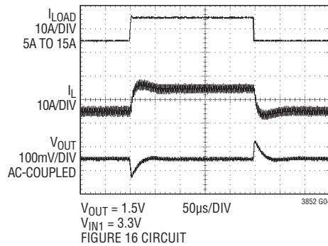
Load Step
